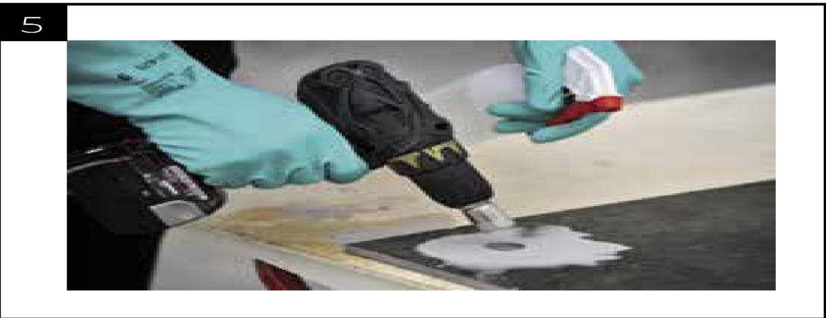
5. Diamond tool for wet drilling
